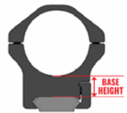
Weaver Rings 30mm / 14mm 050-30-14-V
